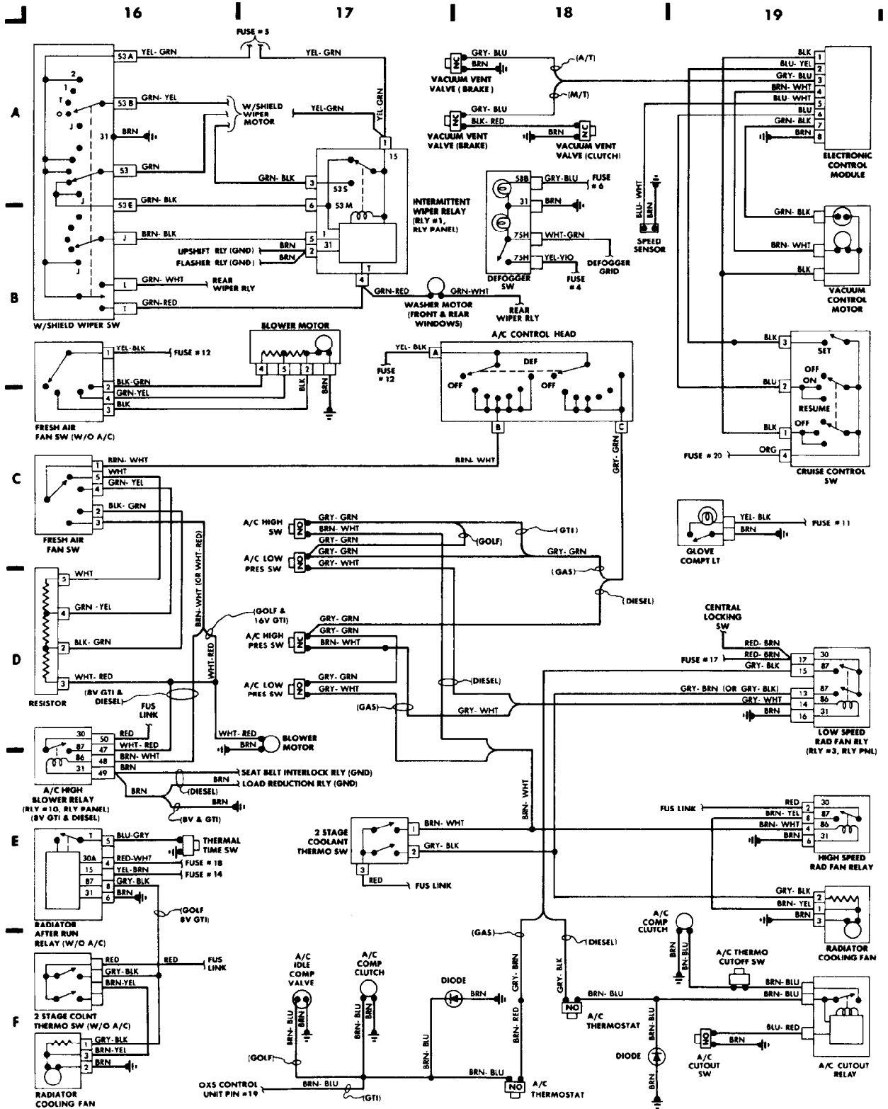
Fig. 5: Underdash (Cont.) & Instrument Panel (Grids 16-19)
