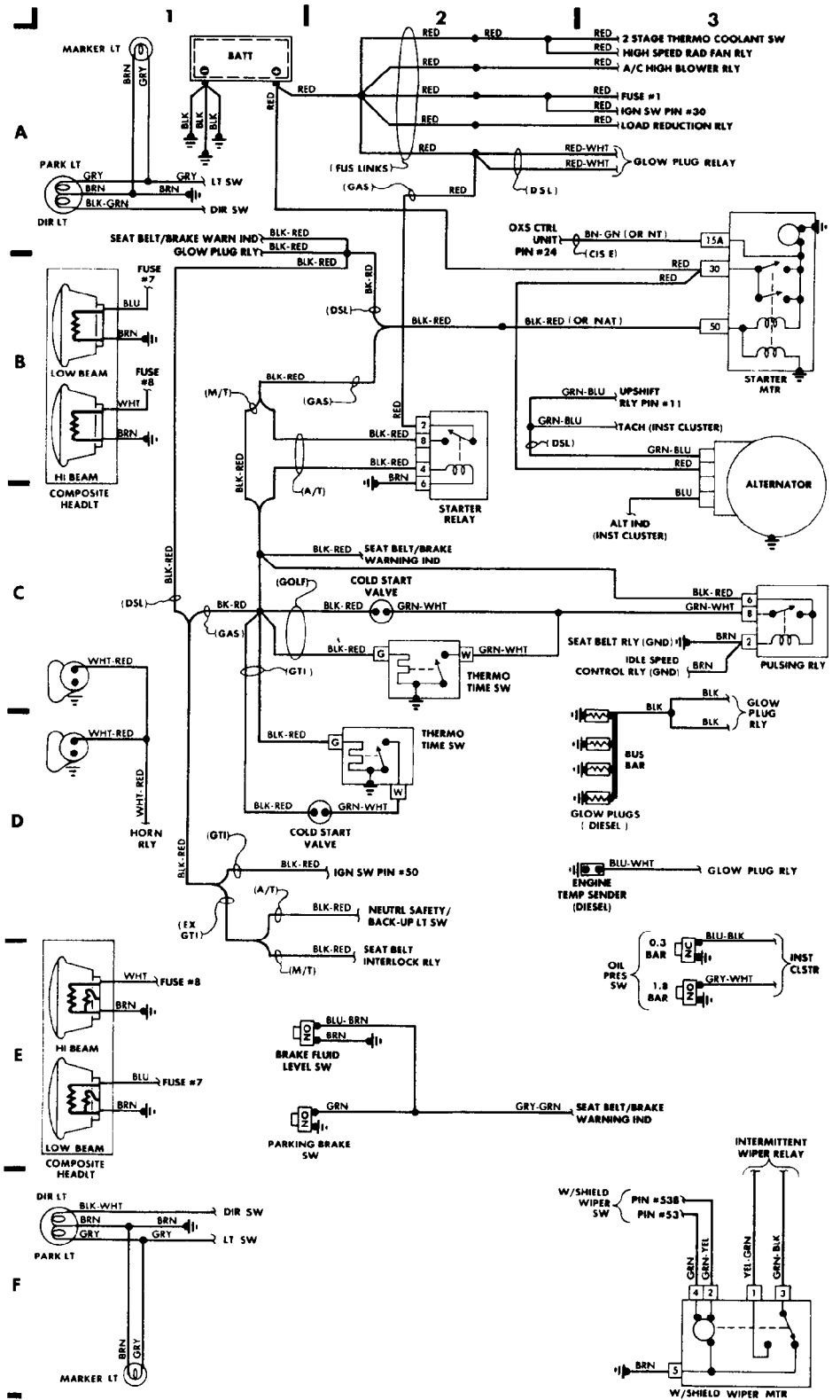
Fig. 1: Engine Compartment (Grids 1-3)
