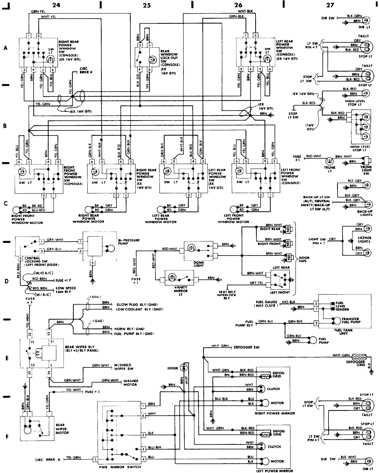
Fig. 7: Rear Compartment & Accessories (Grids 24-27)
