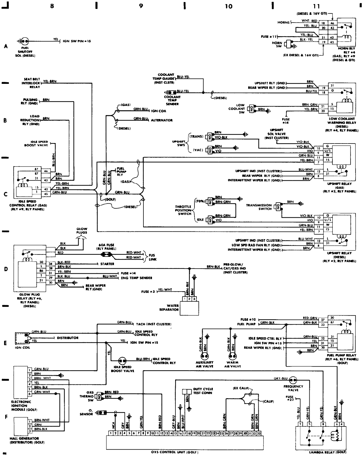
Fig. 3: Engine Compartment (Cont.) & Underdash (Grids 8-11)
