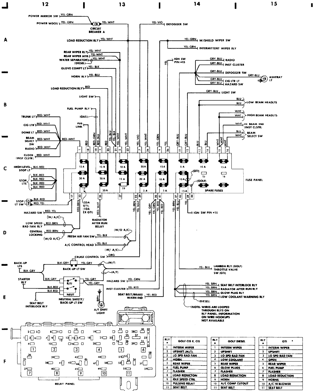
Fig. 4: Underdash (Cont.) & Fuse Block (Grids 12-15)
